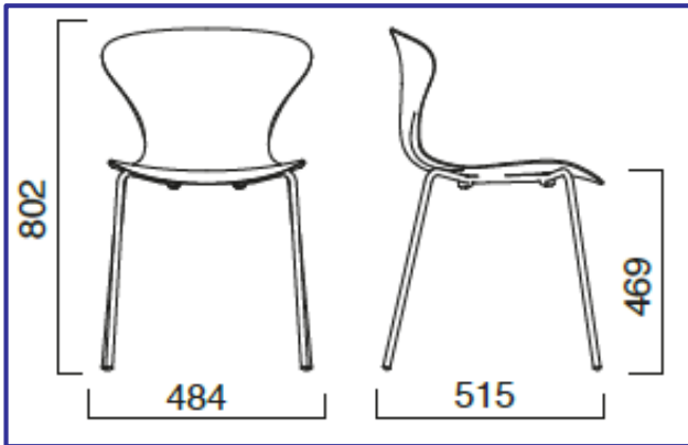
4 Legs
